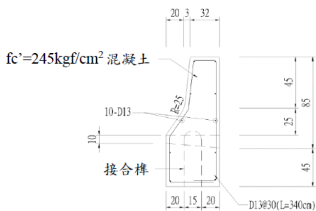
斷面及配筋
